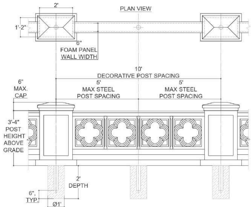
STRUCTURAL SECTION OF A FENCE
